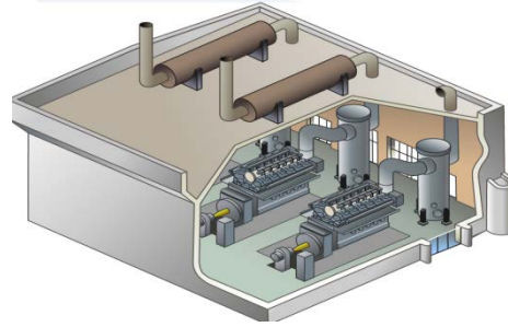
Central generation facility
